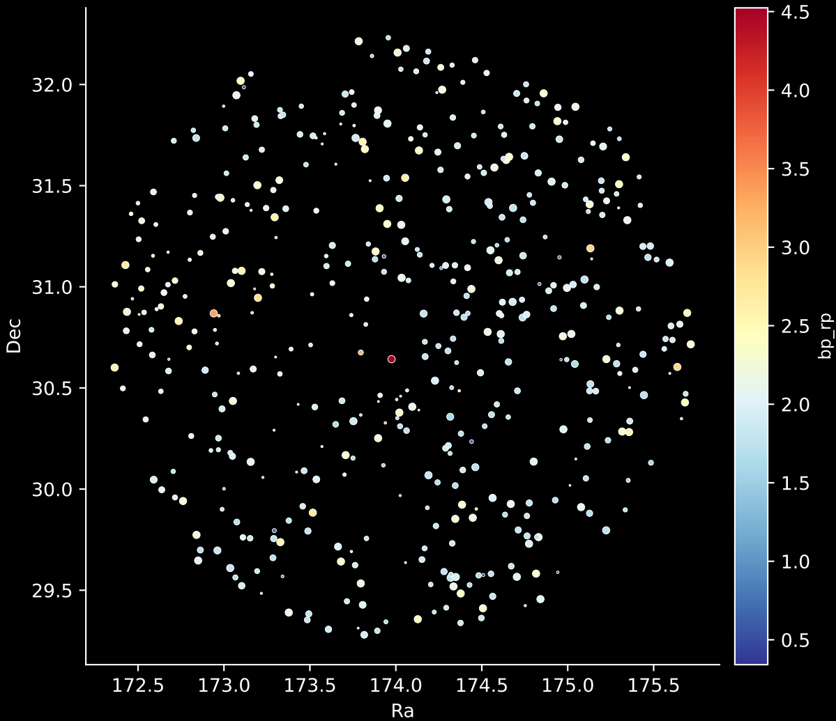
APOGEE DR17 Field: [TAUL1517_btx] Stars: 470
