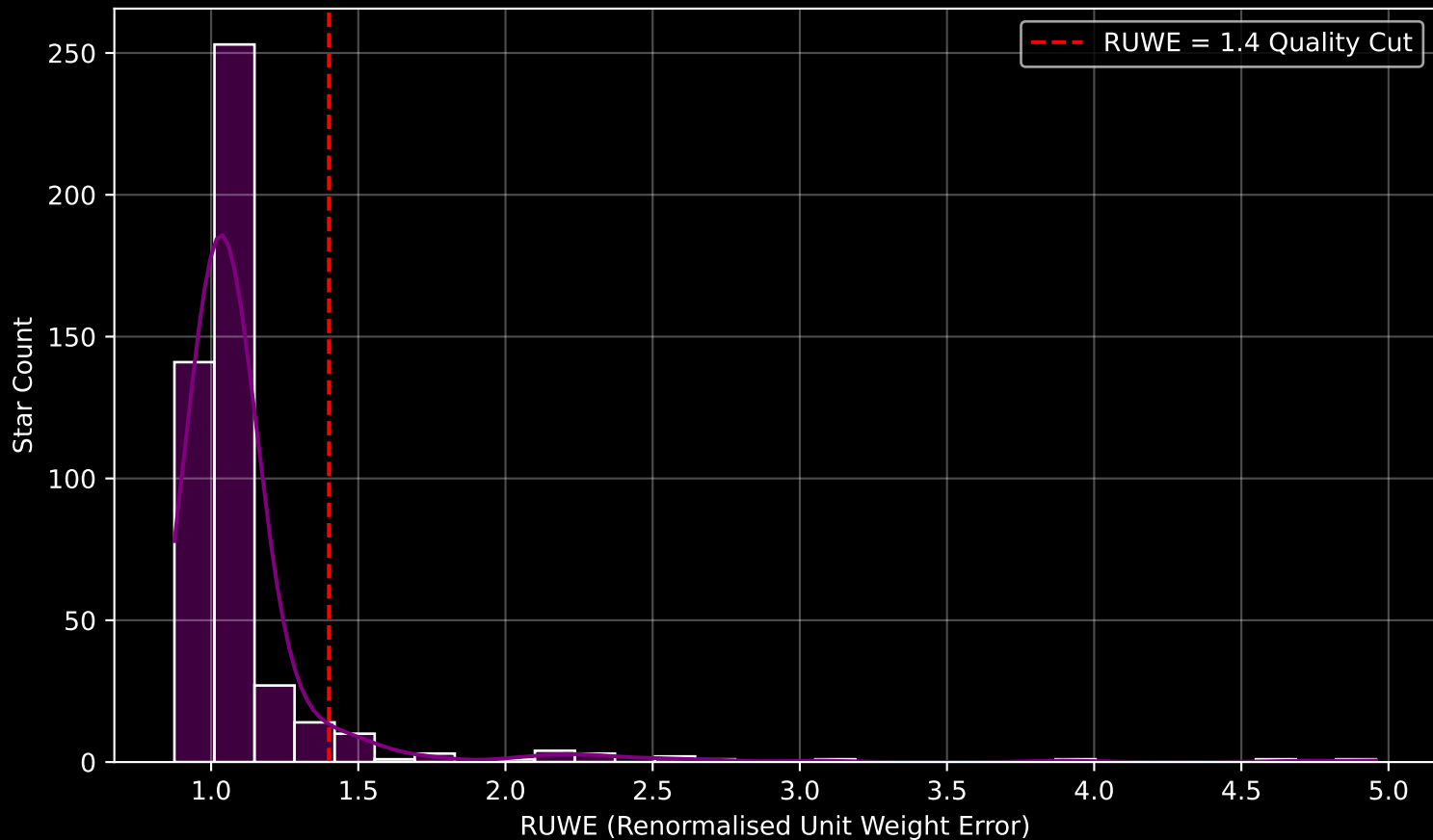
GAPOGEE DR17 Field [TAUL1517_btx] RUWE Distribution (n= 464)
