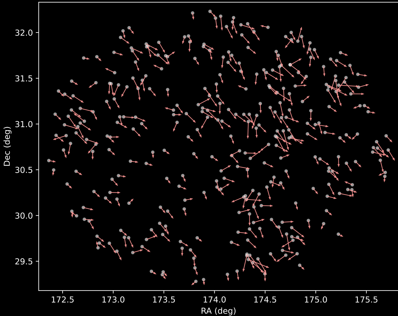
APOGEE DR17 Cluster 7 Proper Motion Vectors (n=331)
