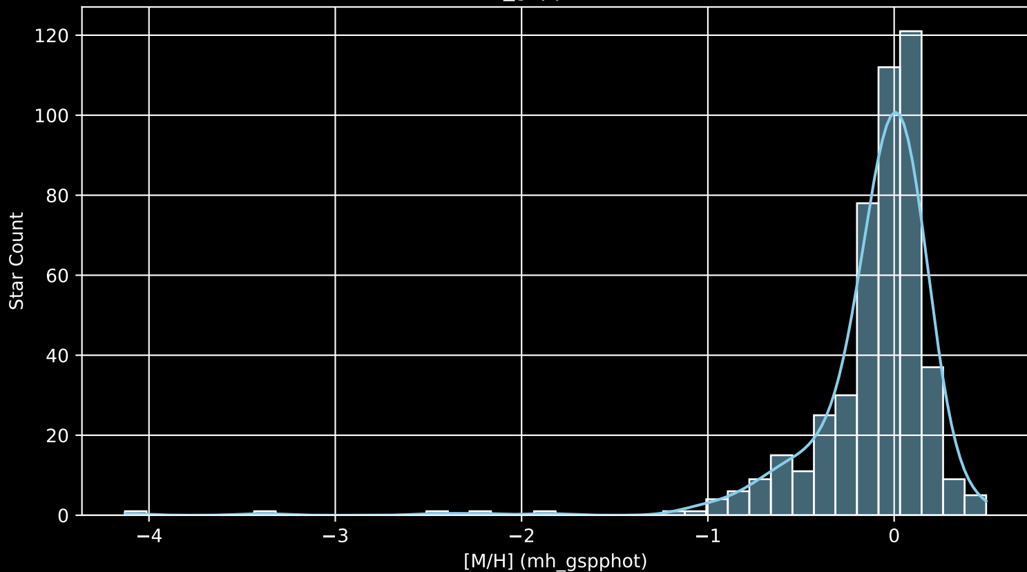
APOGEE DR17 Field: [TAUL1517_btx [M/H] (mh_gspphot) (n= 469)
