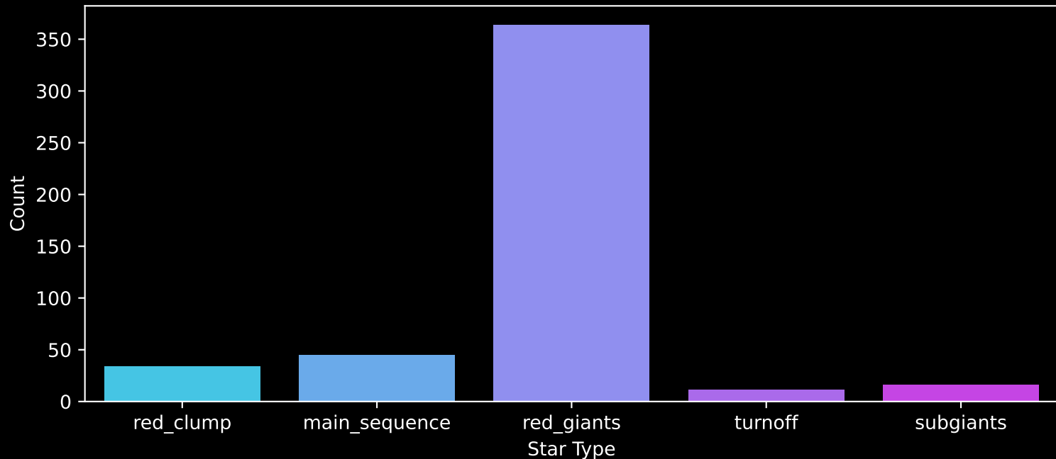
APOGEE DR17 Field: [TAUL1517_btx] Count plot of Star Type
