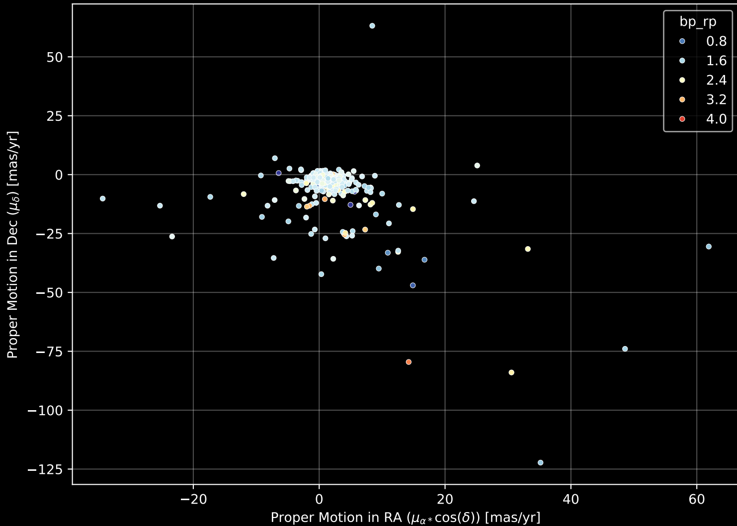
APOGEE DR17 Field: [TAUL1517_btx] Proper Motion Diagram (n= 470)
