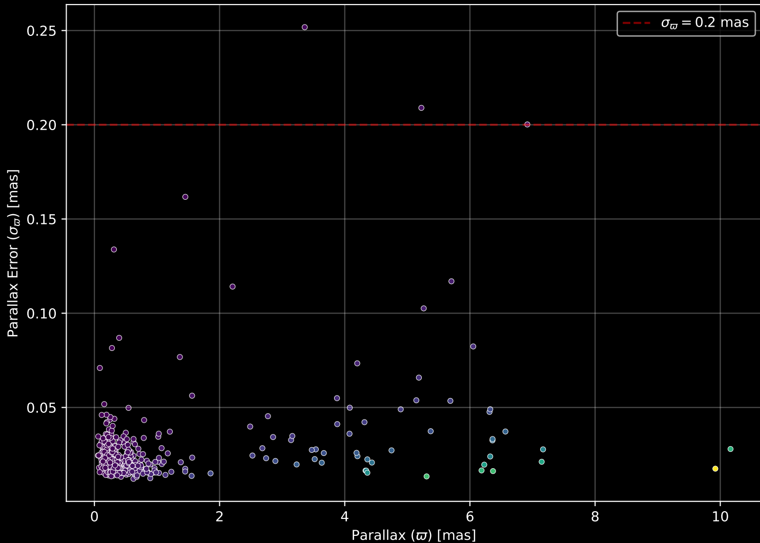
APOGEE DR17 Field: [TAUL1517_btx] Parallax Quality (n= 470)
